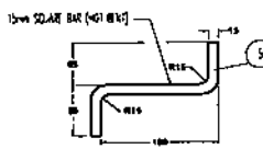
CLIMBING RUNG DETAIL
