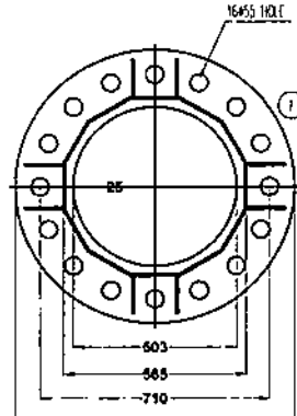
BASE PLATE PLAN
